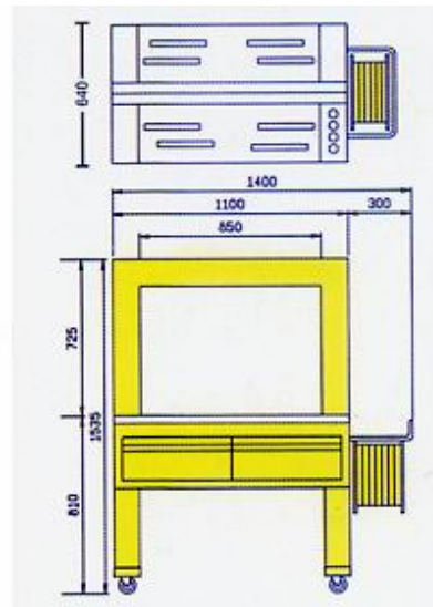
Dimension Diagram
